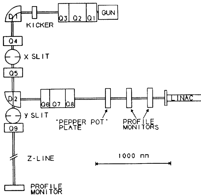
Fig. 2. The ATF injection line
