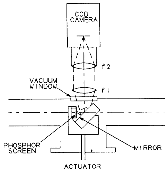
Fig. 1. The ATF beam-profile monitor
