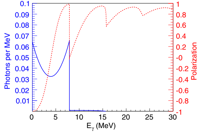
FIG. 3 (color online). Solid line: calculated photon number spectrum per beam electron of undulator radiation integrated over angle, plotted as a function of photon energy E_\gamma for electron beam energy 46.6 GeV, undulator period 2.54 mm and undulator strength parameter K = 0.17 . The peak energy of the first-harmonic (dipole) radiation was 7.9 MeV. Dashed line: longitudinal polarization P_\gamma of the undulator radiation as a function of energy.
