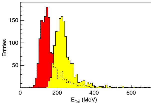
FIG. 4 (color online). Distributions of energy E_{\text{CsI}} observed in the central CsI crystal of the positron polarimeter from individual electron beam pulses with undulator-on (right peak) and undulator-off (left peak). The central positron energy was 6.7 MeV.
