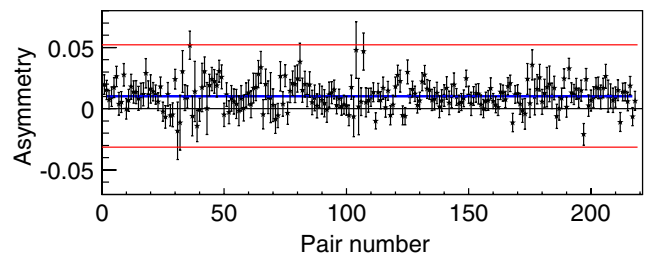
FIG. 5 (color online). Positron-induced asymmetries \delta_{e^+} in the central CsI crystal of the positron polarimeter for 220 pairs of 1500 undulator-on beam pulses with opposite magnetization in the polarimeter. The central positron energy was 6.1 MeV. The average asymmetry was 0.0108, as indicated by the horizontal line.
