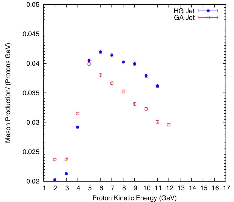
MARS15 (2012)
