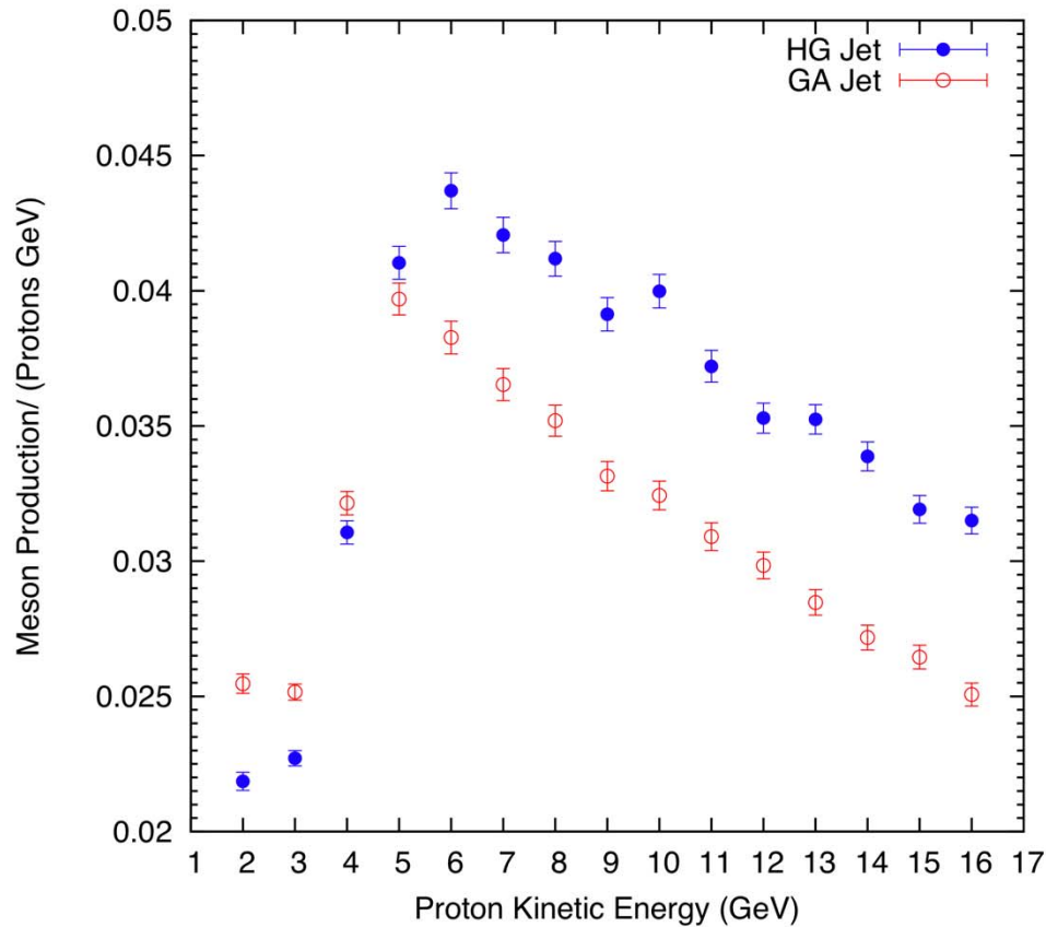
MARS15 (2010)
