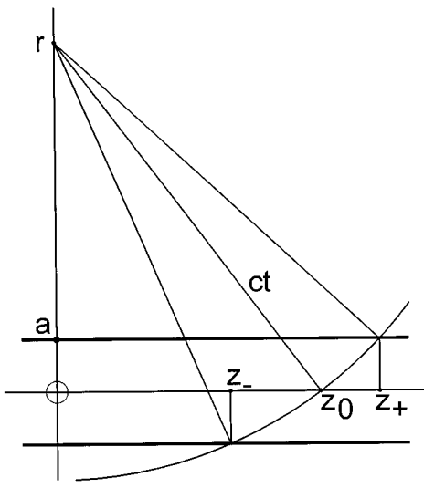
Fig. 1. The fields of a solenoid of radius a concentric with the z axis are observed at the point (r,0,0) in a cylindrical coordinate system. At time t the observer receives radiation emitted at t=0 from points z_+ and z_- on the near and far side of the solenoid, respectively, both of which are distance ct from the observer. The point on the axis at distance ct from the observer is labeled z_0 .
