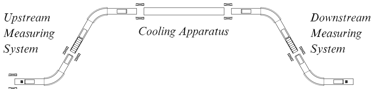
Figure 1: Top view of the layout of the detectors and a 3-T, 30-cm-diameter bent solenoid muon channel surrounding the muon cooling apparatus. Each detector arm is about 8 m long.
