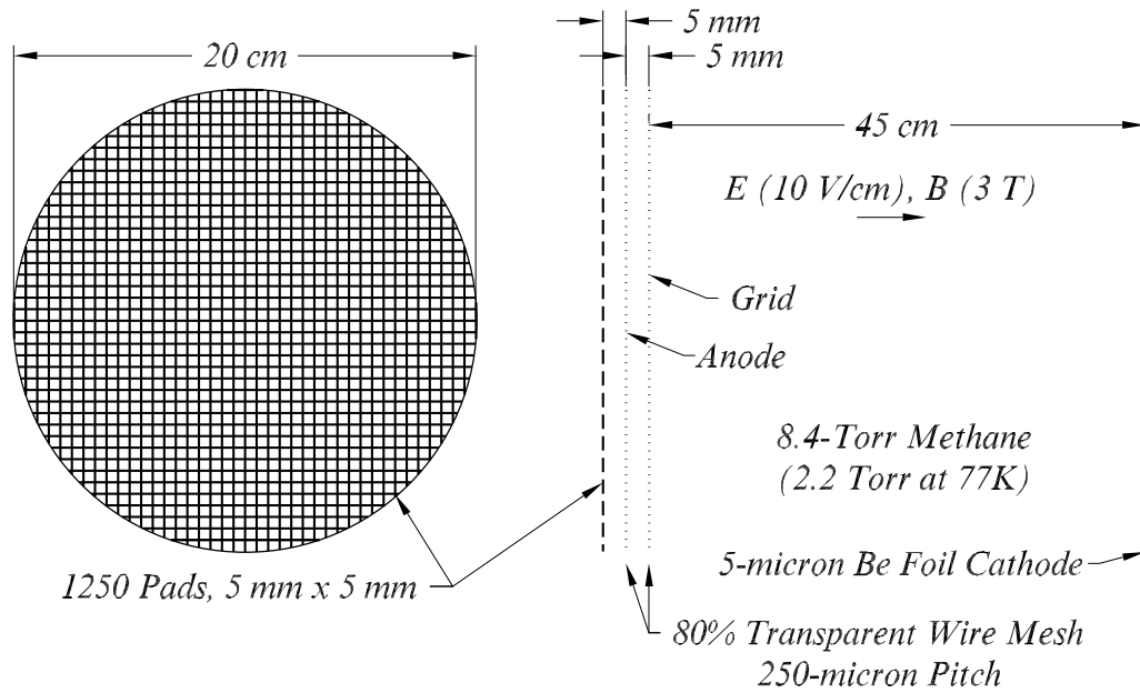
Figure 3: Sketch of the low-pressure time projection chamber.
