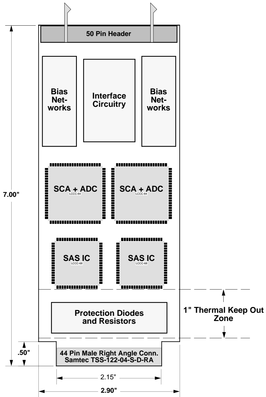
Figure 6: The STAR TPC front-end electronics readout card (FEE).
