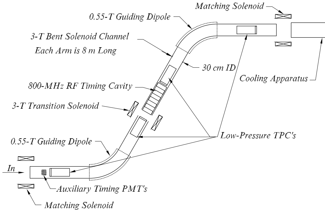
Figure 2: Layout of the 'before' arm of the detector. Vertical guiding dipole fields of 0.55 T are superimposed on the solenoid bends to keep the central trajectory in the horizontal plane.
