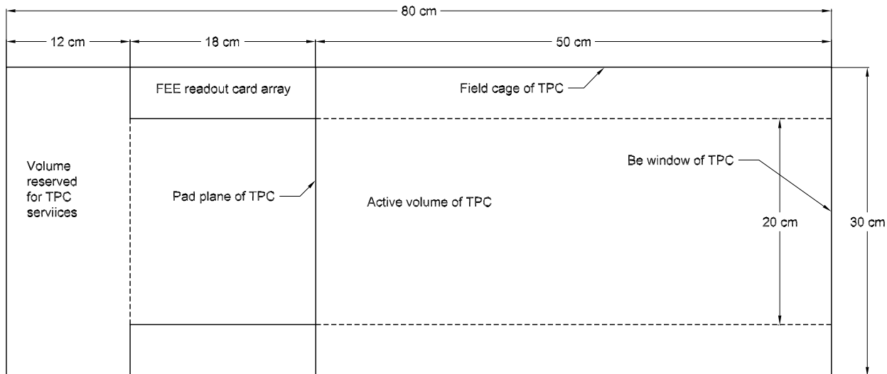
Figure 4: Plan view of the TPC plus front-end electronics.
