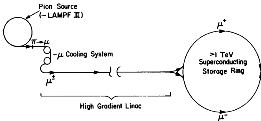
Fig. 5. The \mu linac/storage-ring system.
