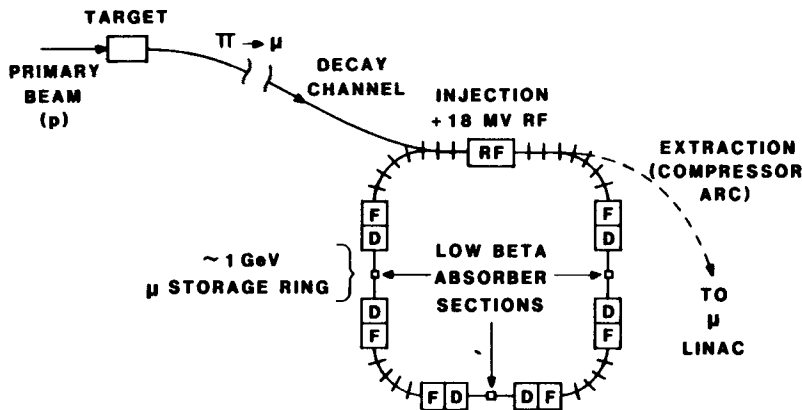
Fig. 3. A muon cooling ring.
