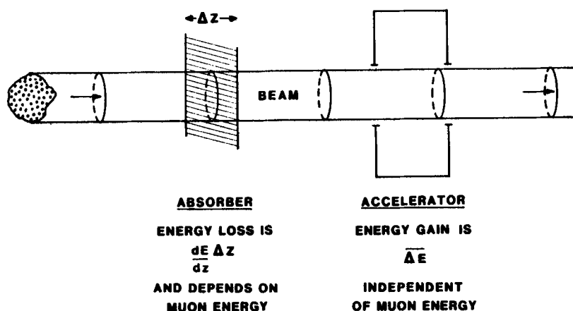
Fig. 1. Sketch of "ionization cooling" principle.
